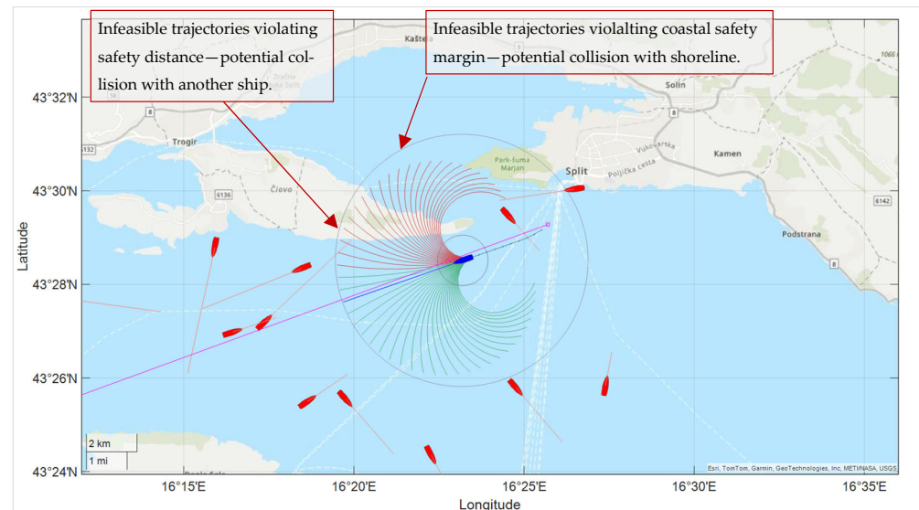
Figure 3. Illustration of simplified MPC implementation, with candidate trajectories color-coded as infeasible (red) or feasible (green). Selected optimal trajectory \tau^* shown in blue.
