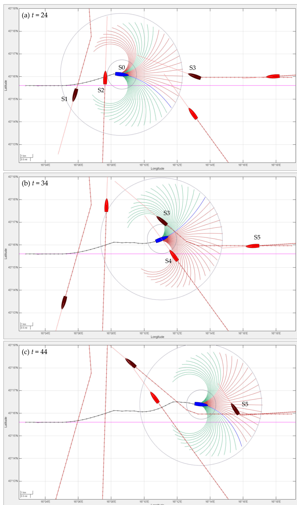
Figure 9. A multi-ship encounter scenario at time steps t = (24, 34, 44) : The own ship (blue, with a black track) avoids multiple surrounding vessels (red) using MPC-based navigation. The candidate trajectories are color-coded as infeasible (red) or feasible (green), and the chosen trajectory is shown in blue. The vessels that alter their heading in accordance with the COLREGs are highlighted in dark red.
